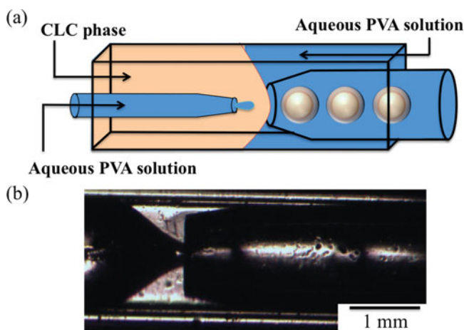
Figure 1. Schematic of the microcapillary geometry for generating CLC core-shell microspheres. (a) The geometry required the outer phase to be immiscible with the middle phase, which is in turn immiscible with the inner phase. (b) Optical micrograph of the microfluidic device.
