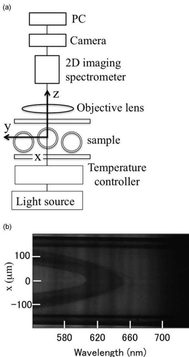
Figure 3. Two-dimensional (2-D) transmittance spectra of a CLC core-shell microsphere for mapping of the spectra on the shell surface. (a) Experimental setup of the 2-D transmittance spectroscopy. (b) 2-D transmittance spectra of a CLC core-shell microsphere with the outer diameter of 353\ \mu\text{m} and shell thickness of 31\ \mu\text{m} .
