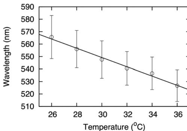
Figure 4. Temperature dependence of the center of the PBG of the CLC core-shell microspheres at x = y = 0 . Error bars denote the width of the PBG at each temperature.
